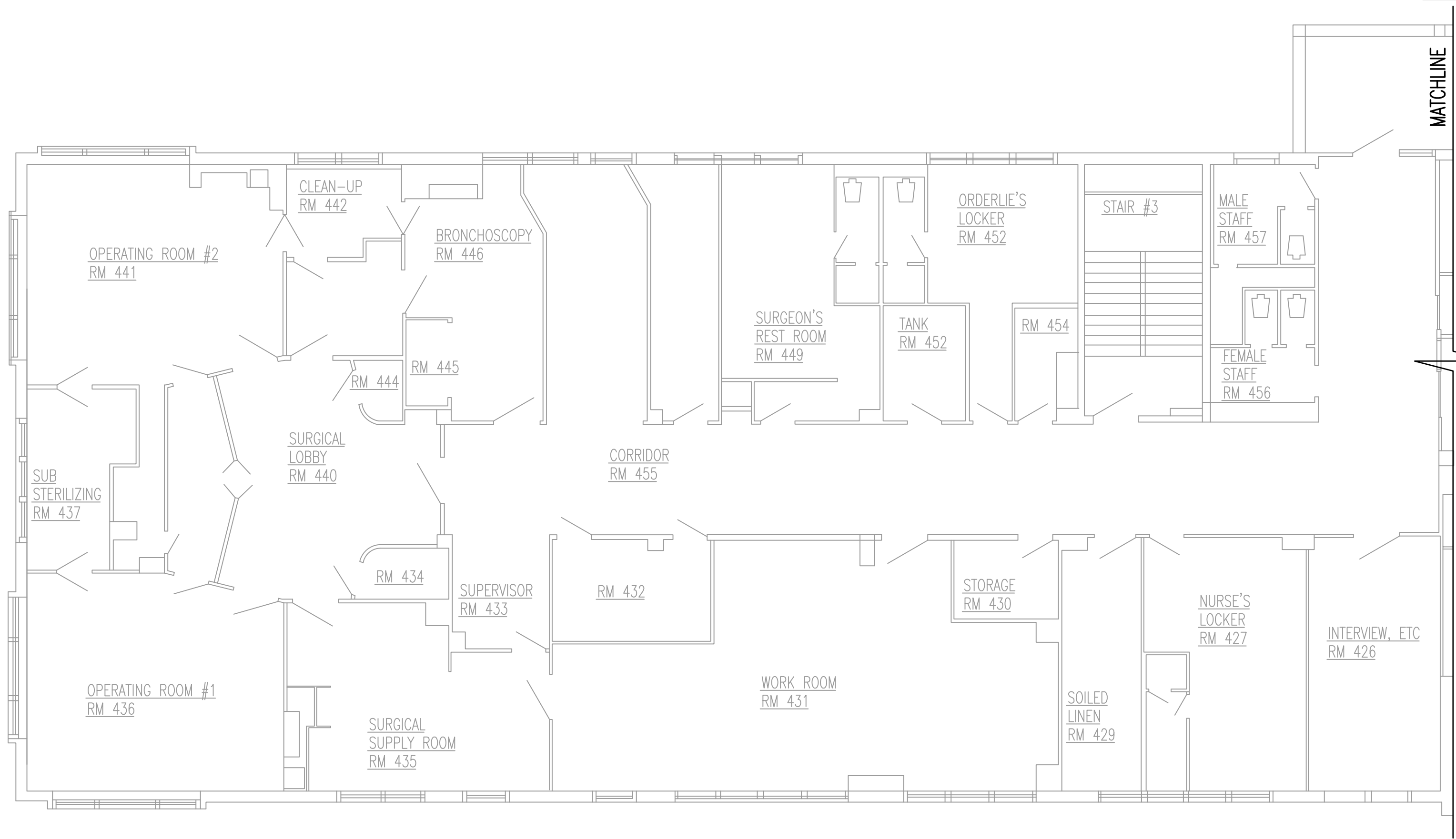
YOUNG BUILDING - 4TH FLOOR PLAN SCALE: 1/8" = 1'-0"
