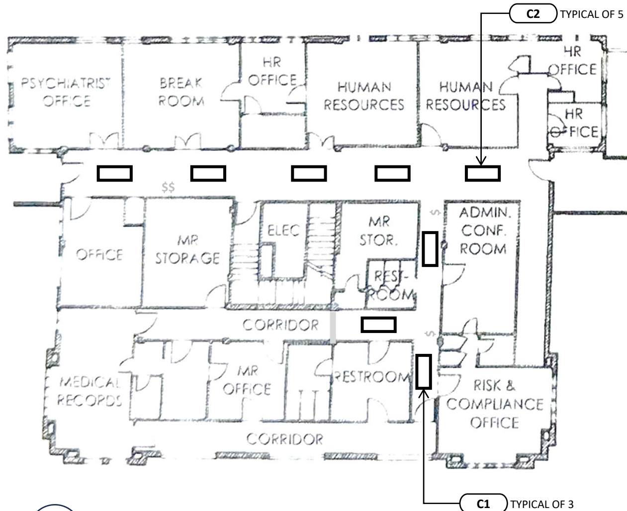
SECOND FLOOR LIGHTING PLAN NOT TO SCALE
