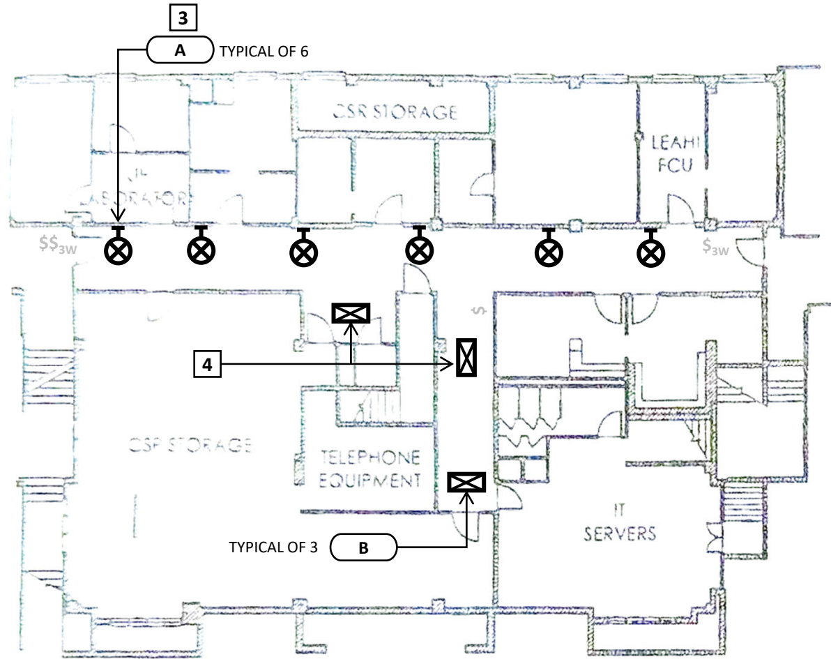
BASEMENT LIGHTING PLAN NOT TO SCALE
