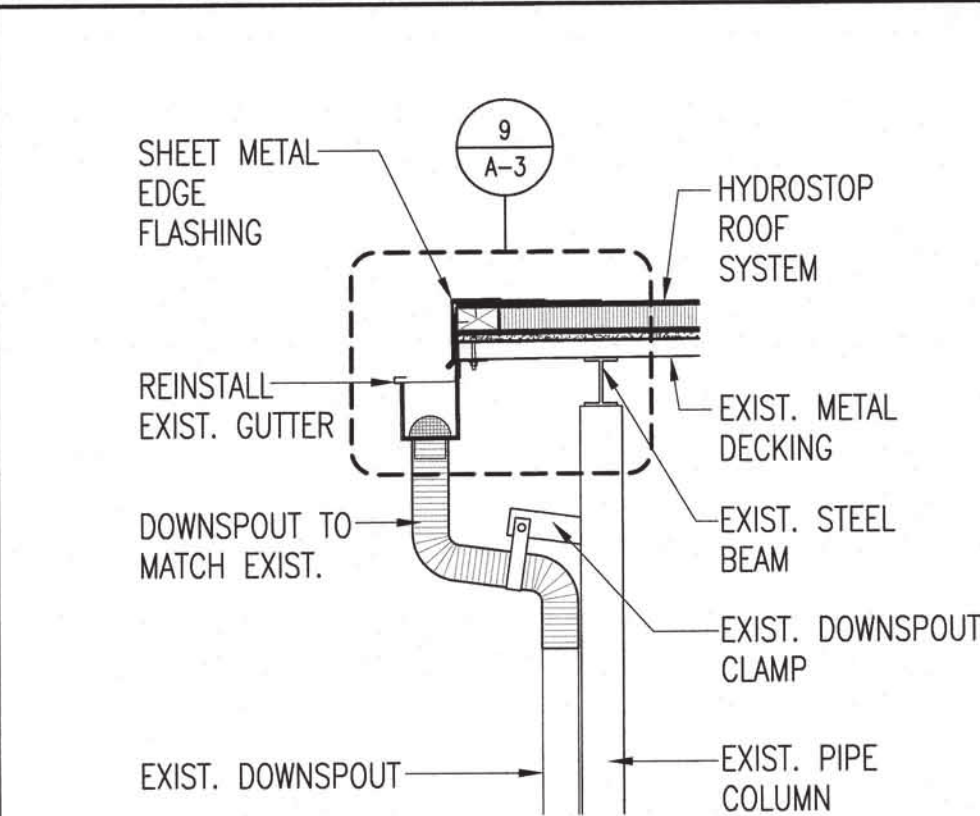
4 ROOF OVERHANG DETAIL A-3 SCALE: 3/4"=1'-0"
