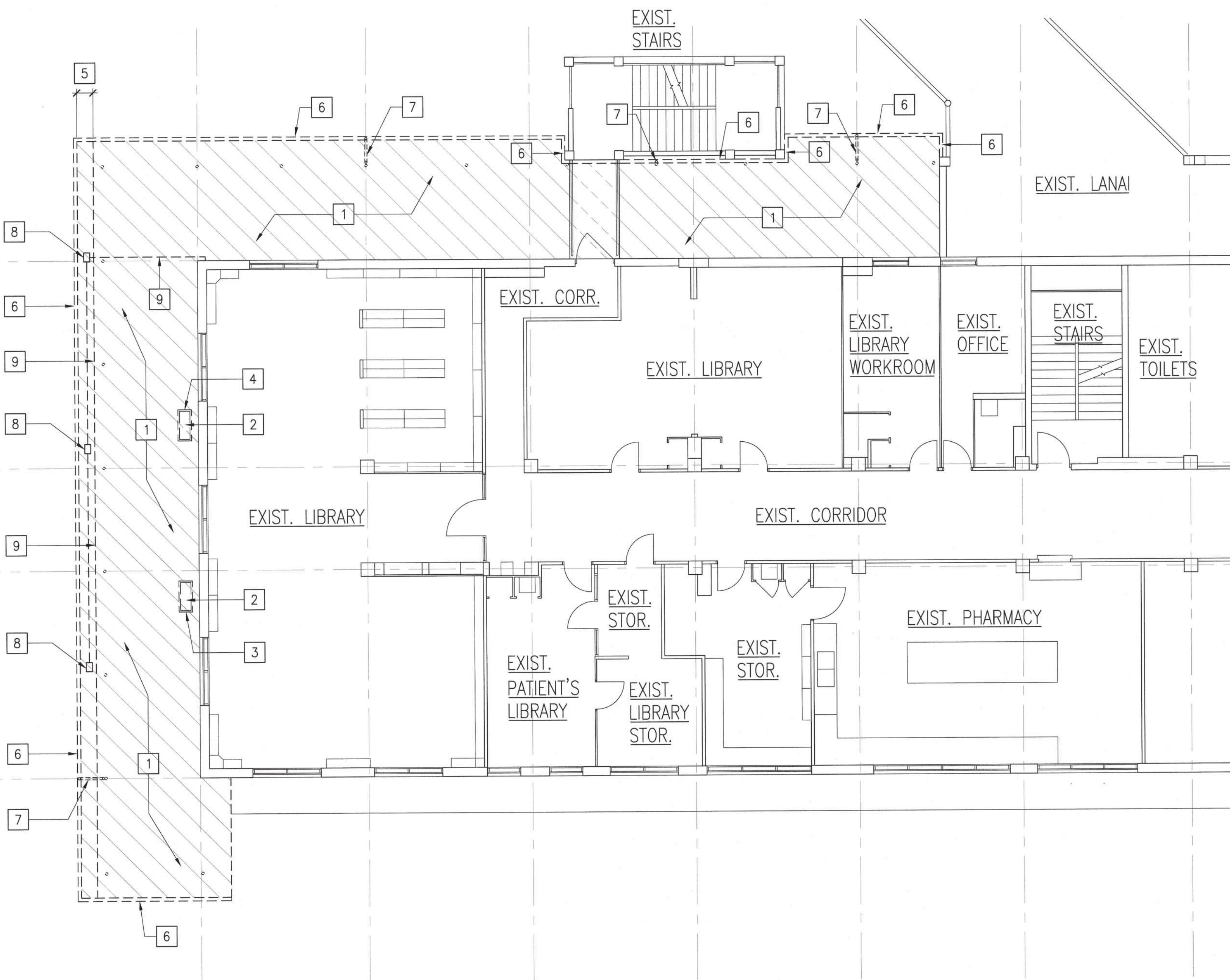
PARTIAL EXISTING SECOND FLOOR PLAN AND DEMOLITION LOWER ROOF PLAN SCALE: 1/8" = 1'-0"
