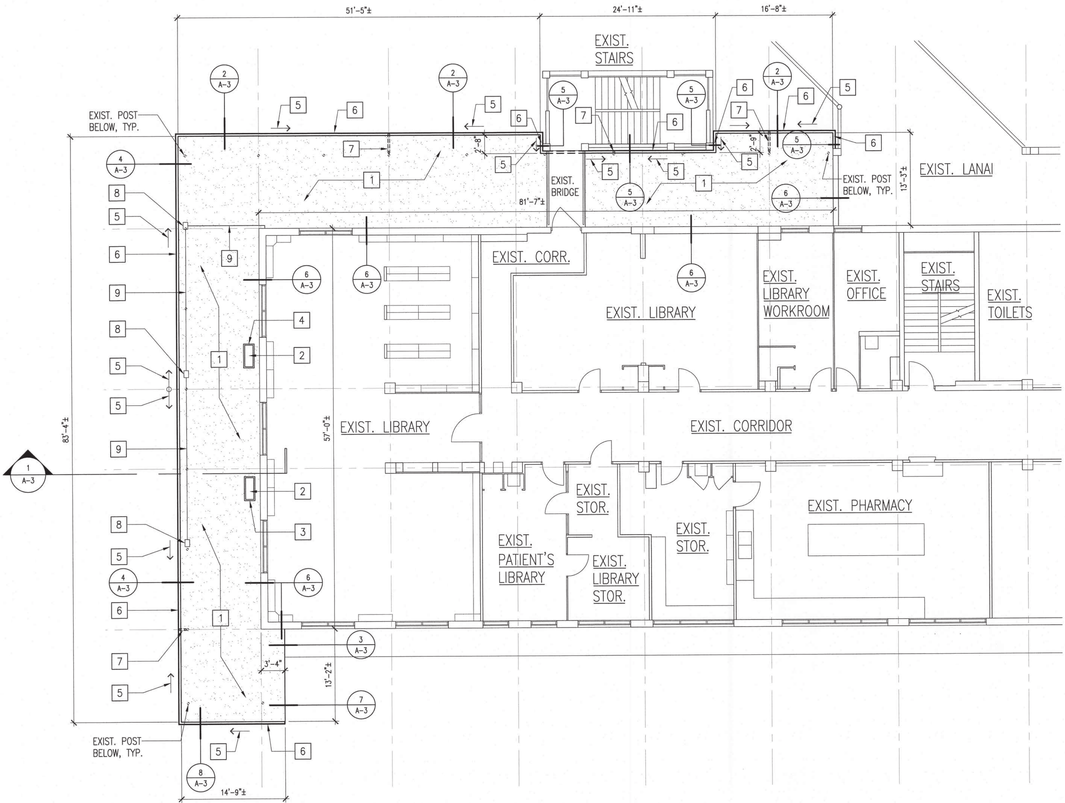
PARTIAL EXISTING SECOND FLOOR PLAN AND NEW LOWER ROOF PLAN SCALE: 1/8" = 1'-0"
