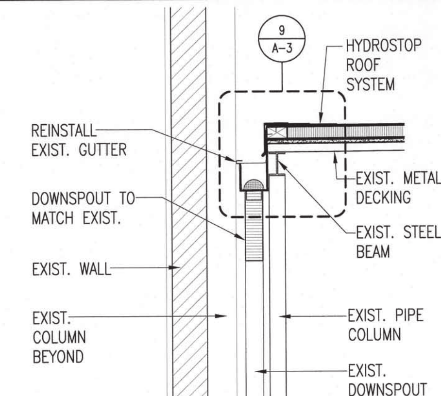
5 ROOF OVERHANG DETAIL A-3 SCALE: 3/4"=1'-0"
