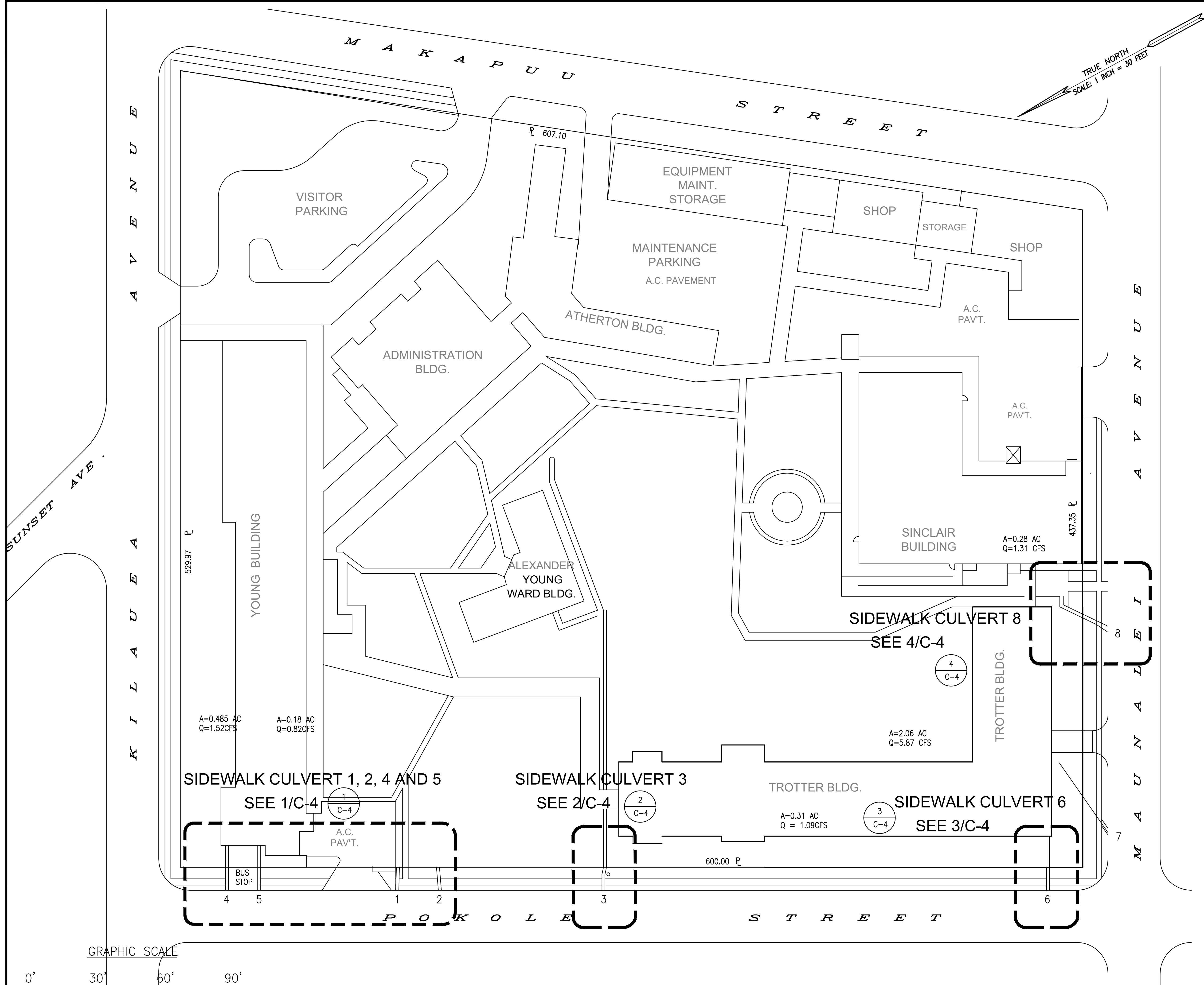
LEAHI HOSPITAL GENERAL SITE PLAN SCALE: 1" = 30'-0"
